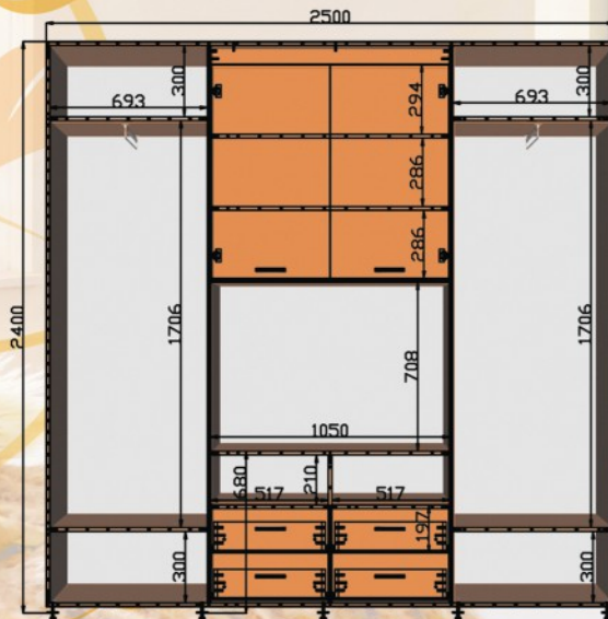
ШК ТВ4 2500x450/600x2400
