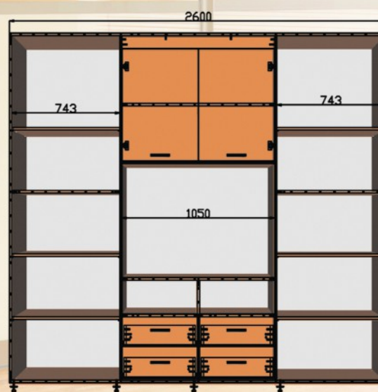
ШК ТВ5 2600x450/600x2200
