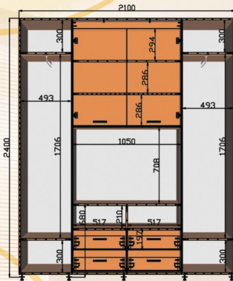
ШК ТВ4 2100x450/600x2400
