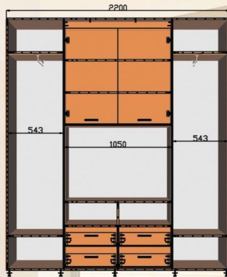
ШК ТВ4 2200x450/600x2400
