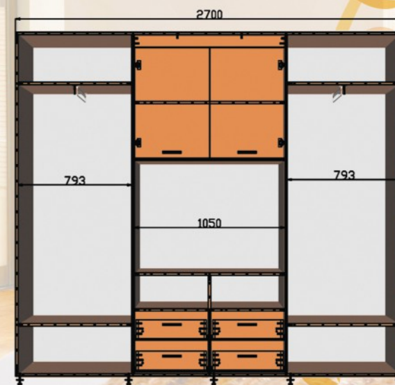
ШК ТВ4 2700x450/600x2200
