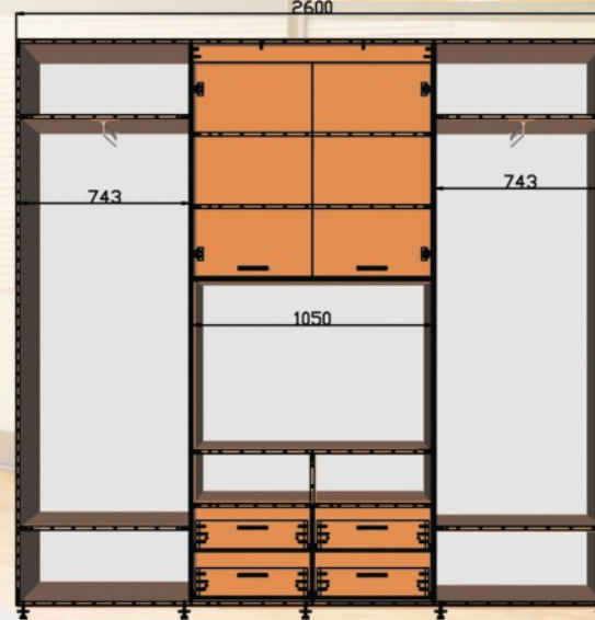
ШК ТВ4 2600x450/600x2400
