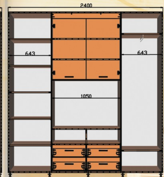
ШК ТВ1 2400x450/600x2400
