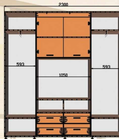
ШК ТВ4 2300x450/600x2200
