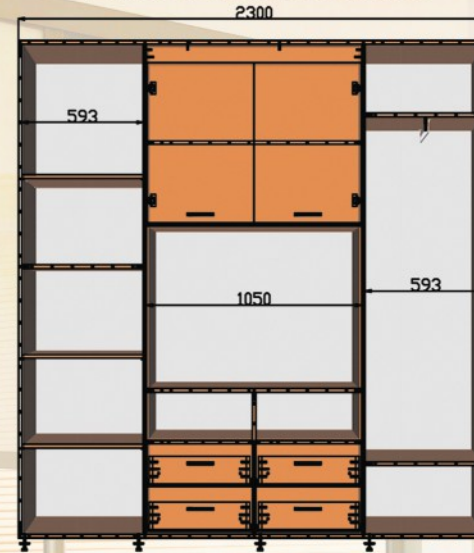
ШК ТВ1 2300x450/600x2200
