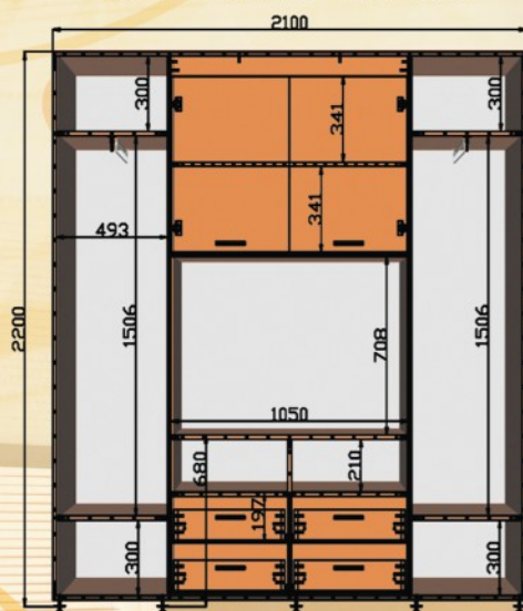
ШК ТВ4 2100x450/600x2200
