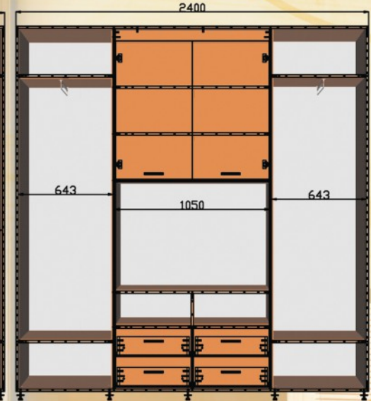
ШК ТВ4 2400x450/600x2400
