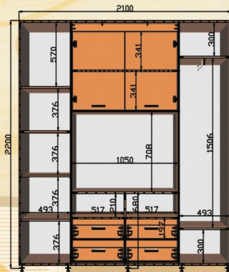
ШК ТВ1 2100x450/600x2200
