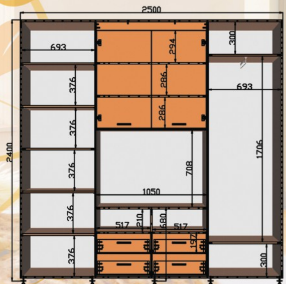
ШК ТВ1 2500x450/600x2400
