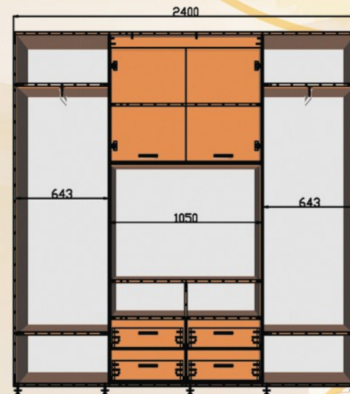
ШК ТВ4 2400x450/600x2200
