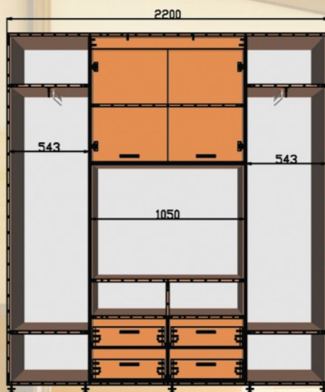
ШК ТВ4 2200x450/600x2200
