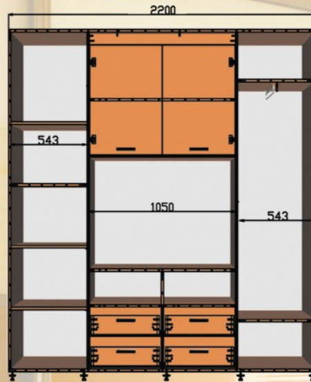
ШК ТВ1 2200x450/600x2200
