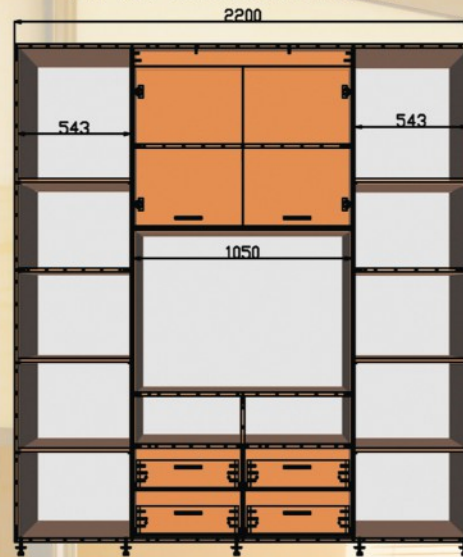
ШК ТВ5 2200x450/600x2200
