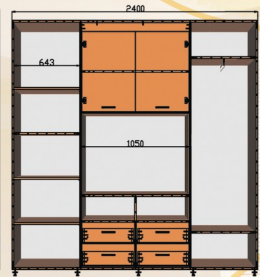
ШК ТВ1 2400x450/600x2200
