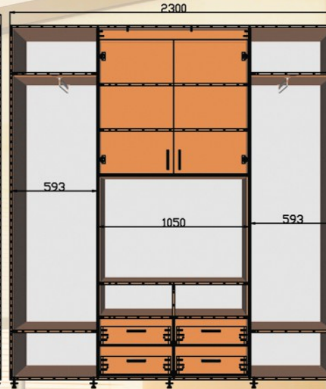
ШК ТВ4 2300x450/600x2400
