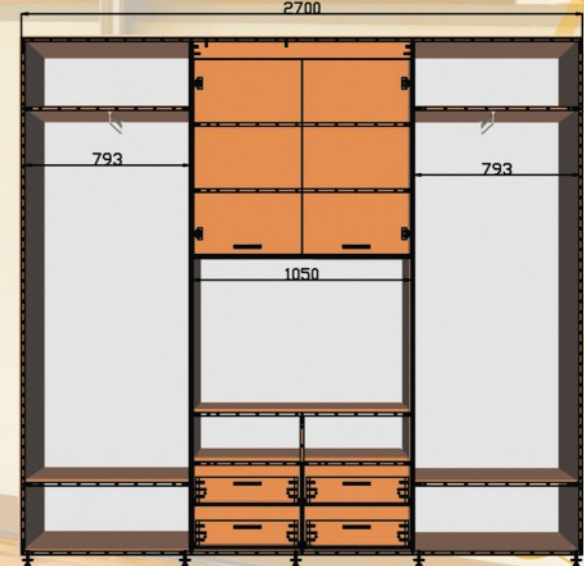
ШК ТВ4 2700x450/600x2400
