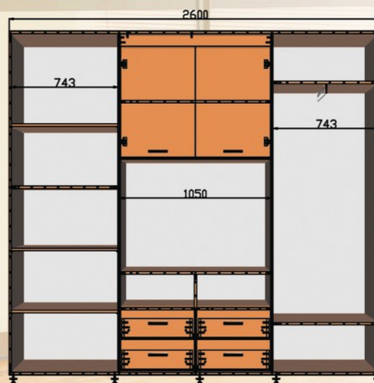
ШК ТВ1 2600x450/600x2200
