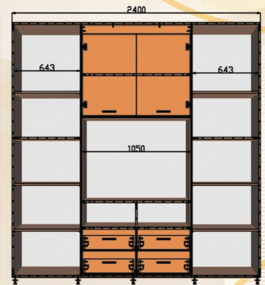
ШК ТВ5 2400x450/600x2200
