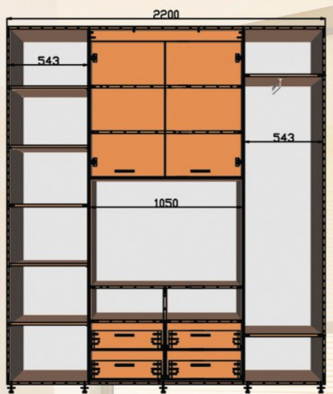
ШК ТВ1 2200x450/600x2400
