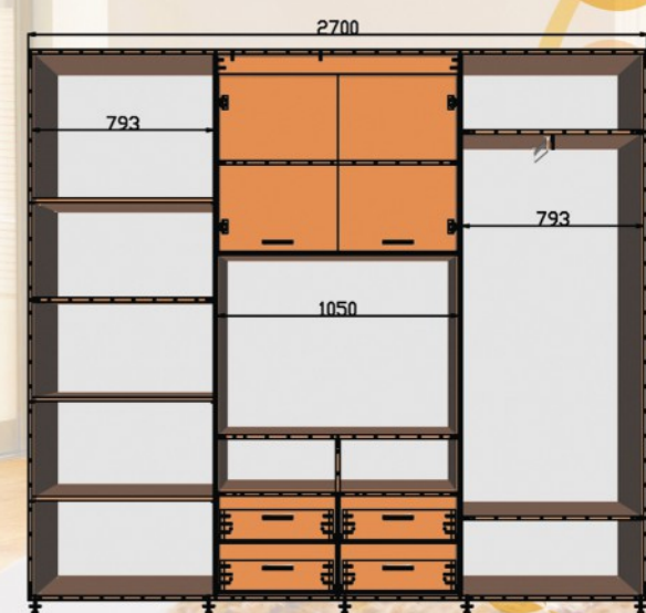
ШК ТВ1 2700x450/600x2200
