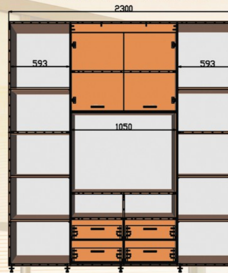
ШК ТВ5 2300x450/600x2200
