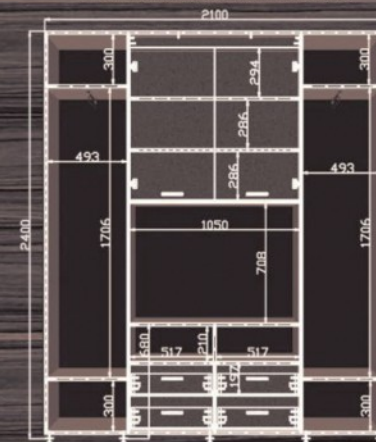
ШК ТВ4 2100x450/600x2400
