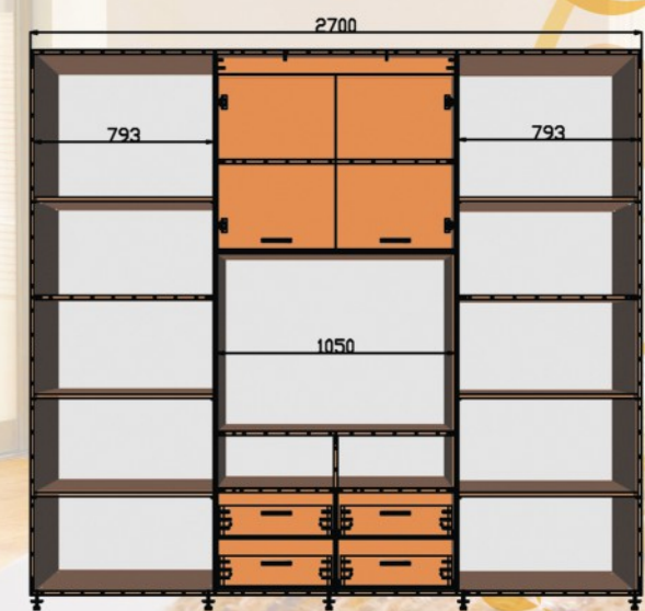
ШК ТВ5 2700x450/600x2200
