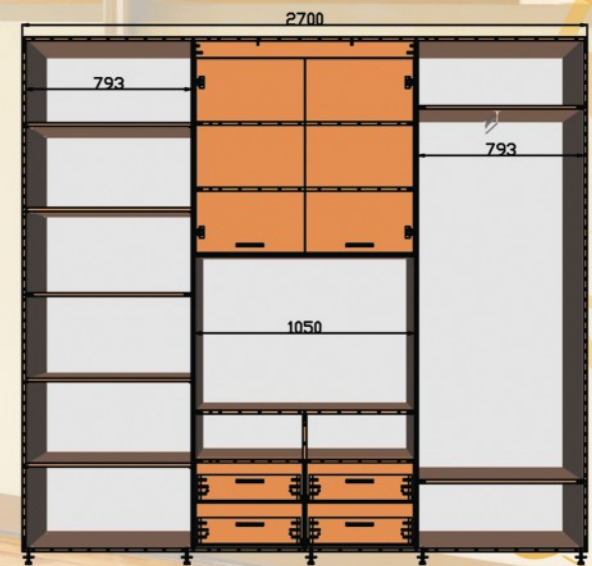
ШК ТВ1 2700x450/600x2400
