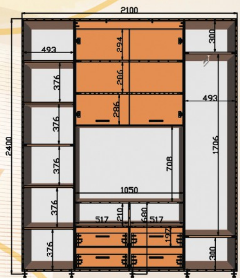
ШК ТВ1 2100x450/600x2400
