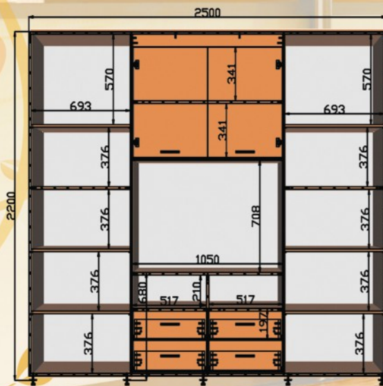
ШК ТВ5 2500x450/600x2200
